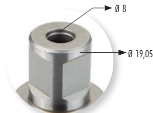
DOUBLE WELDON SHANK
